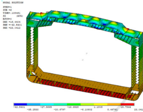
Figure 3: Working Stress of FSO in Hogging.
