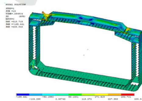
Figure 7: Deformation of FSO at Collapse.
