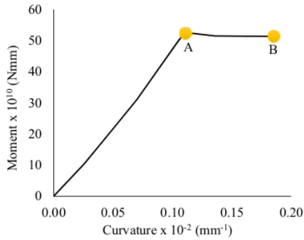
Figure 8: Moment-Curvature of FPSO in Hogging.
