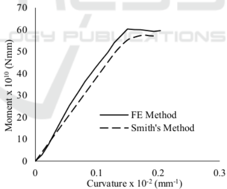
Figure 12: Comparison of Moment-Curvature Relationship.
