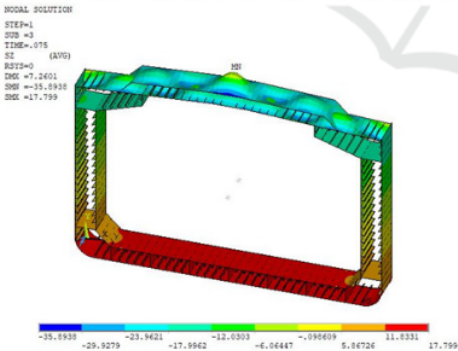
Figure 4: Working Stress of FPSO in Hogging.
