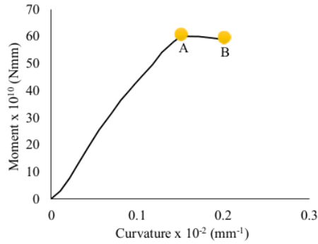
Figure 5: Moment-Curvature of FSO in Hogging.
