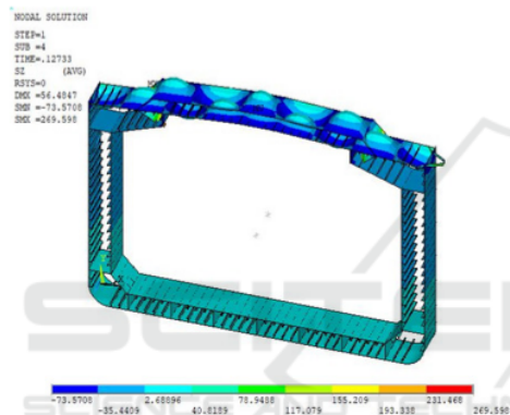
Figure 9: Deformation of FPSO at Ultimate Strength.
