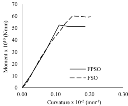
Figure 11: Moment-Curvature Relationship.
