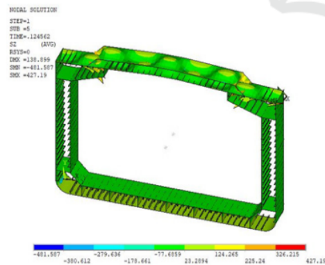
Figure 10: Deformation of FPSO at Collapse.
